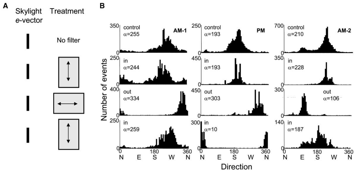
Figure 2. Flight Orientation of Individual Butterflies in Which the Plane of Polarized Skylight Was Varied
